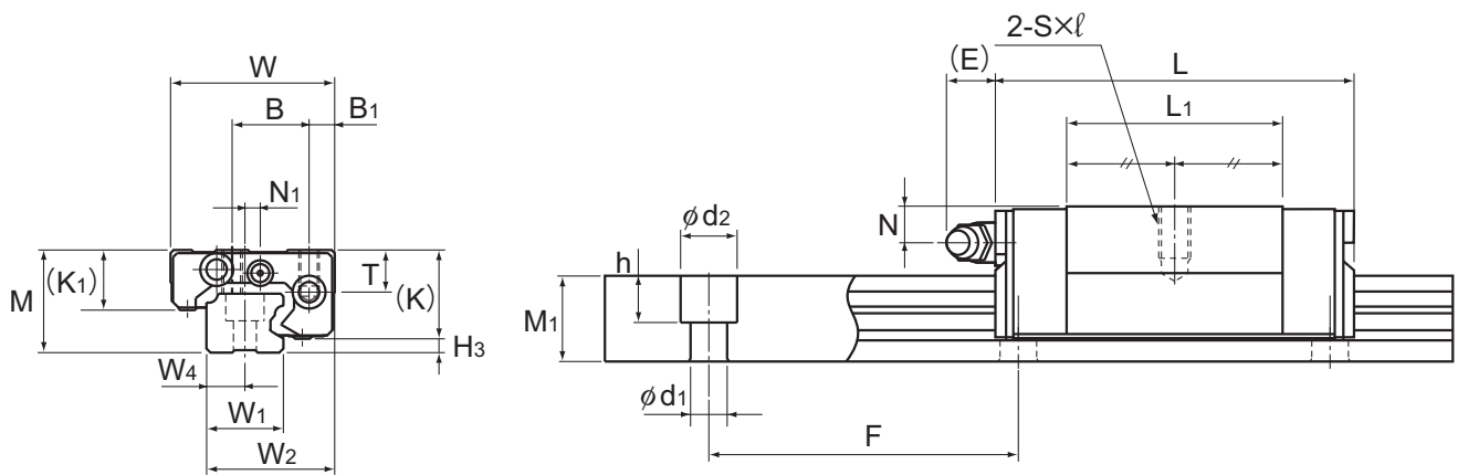
Model GSR15T/V
