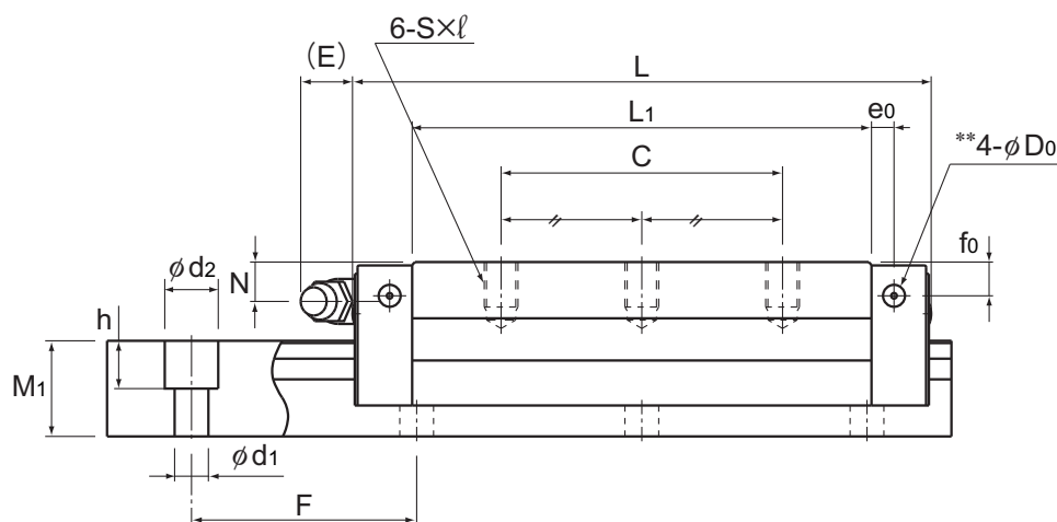
Model SNS-LR
