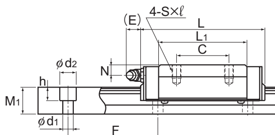
Model SR-W
