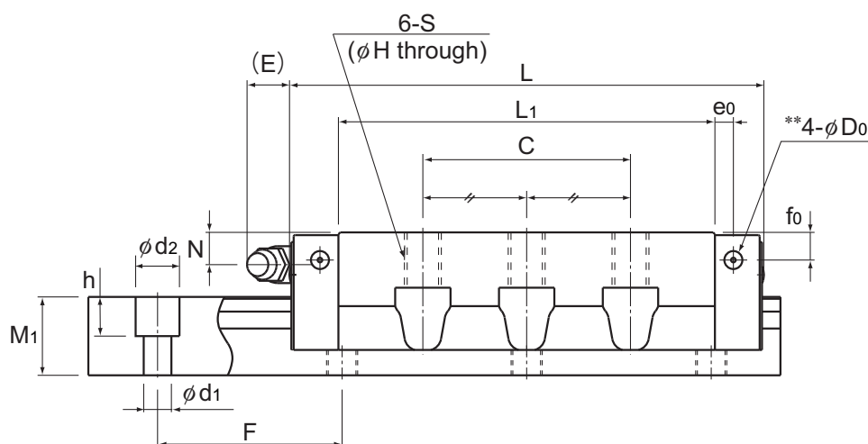
Model SNS-LC
