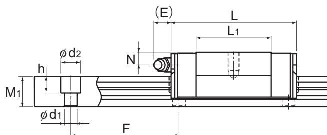
Model GSR25V-R
