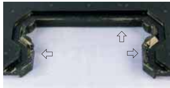
No. 1: without LaCS - lip fractured at 1,700 km
