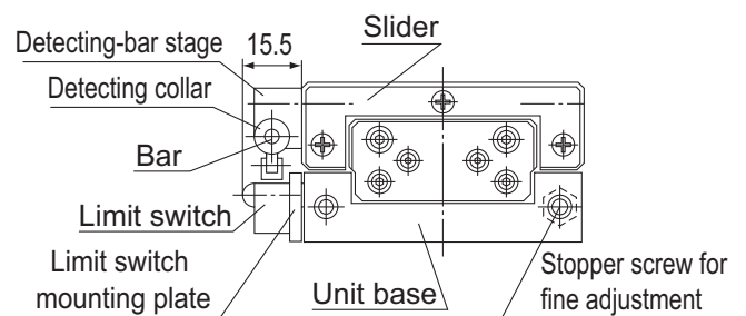
Fig.3 Unit Base and Limit Switch Installation
