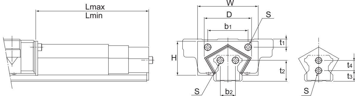
Models HSR25 and 30
