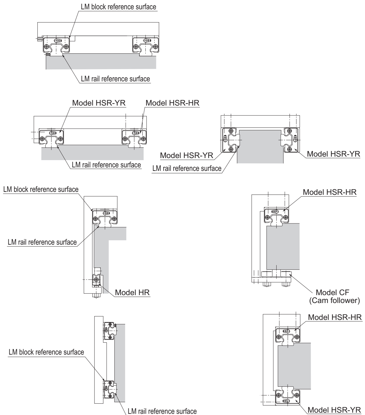
Double-rail configuration
