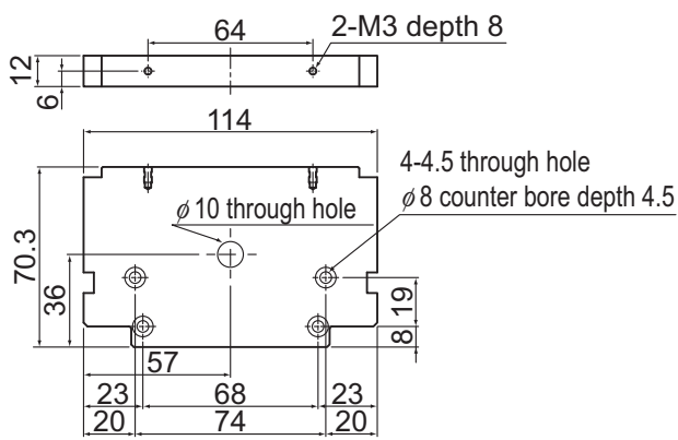
Model GL15
