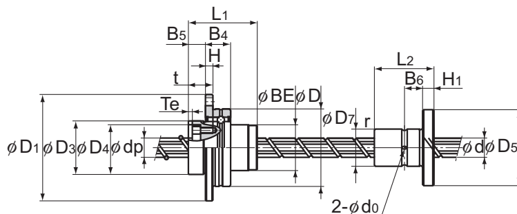
Models NS 0812A and 1015A
