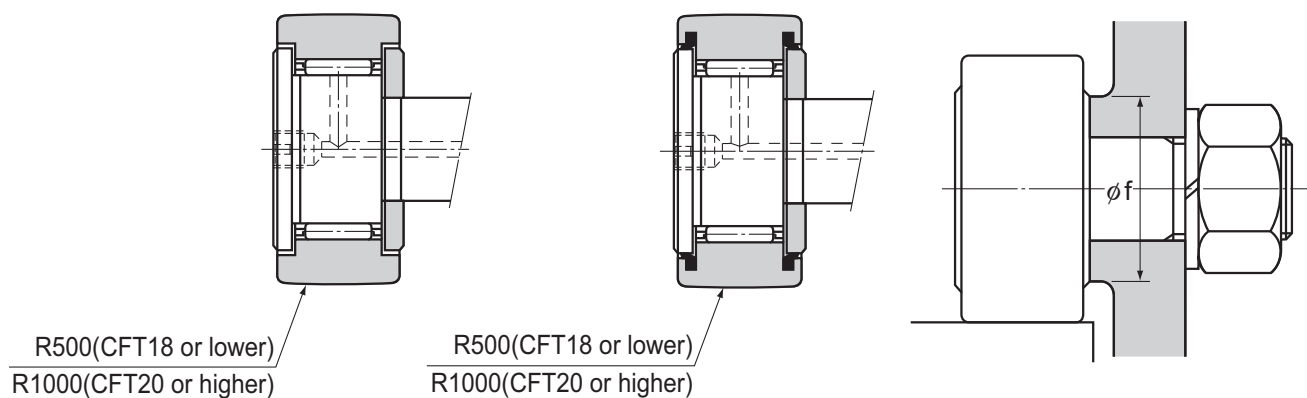
Model CFT-R
