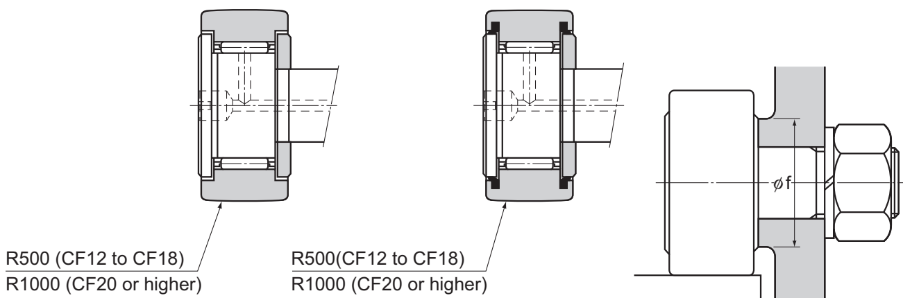
Model CF-R-B
