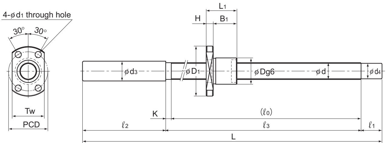
Model MDK
