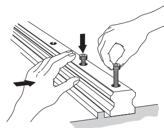
Fig.4 Checking with the Bolt for an Allowance
