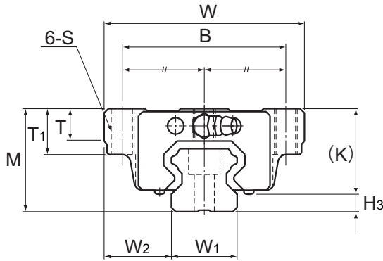
Models HSR20 to 35CA/HA/CAM/HAM
