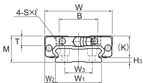
Models HRW17 and 21CR/CRM
