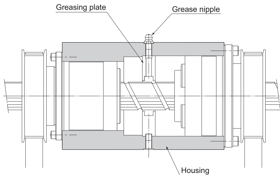
Fig.6 Lubrication Methods
