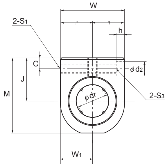
Model SH
