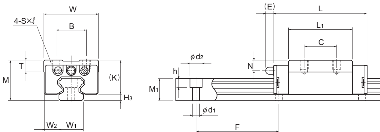
Model HSR12RM
