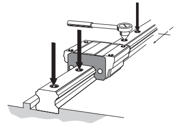
Fig.6 Fully Fastening the Mounting Bolts
