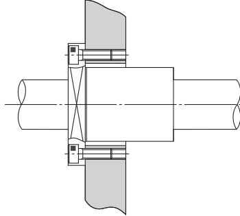
Mounted via a flange only
