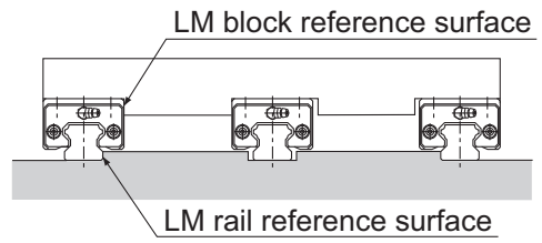
Triple-rail configuration
