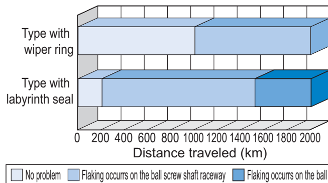
Change in the ball after traveling 2000 km
