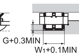
Model LRA or LRA-Z
