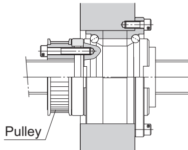
Inverted flange
