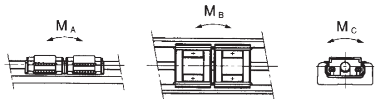
With double short nut blocks (type D)
