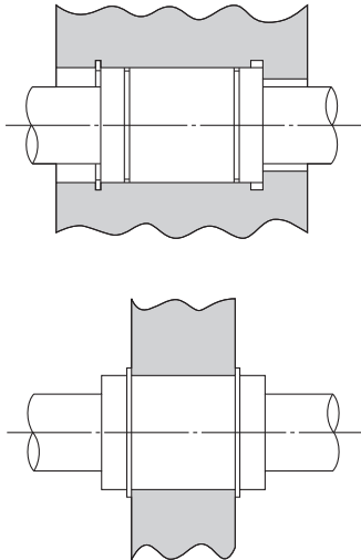
Fig.1 Snap Ring
