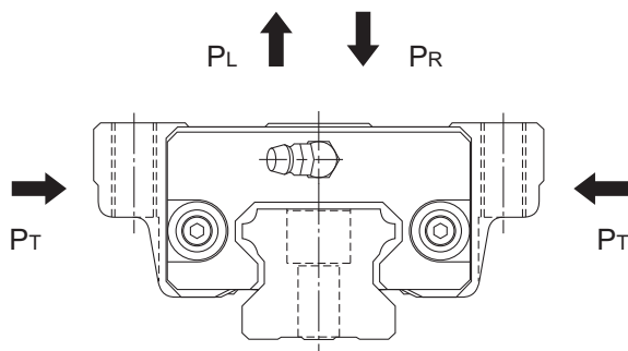
Fig.3 Model HSR-M1
