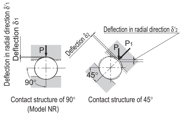
Fig.1 Deflection under a Radial Load
