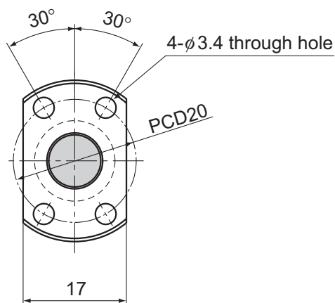
X-X arrow view
