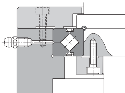
b. Inner ring rotating in the swiveling unit (with seals attached)
