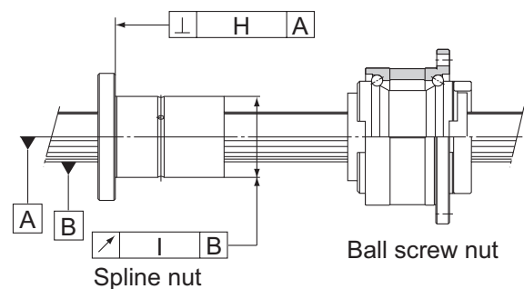
Model NS
