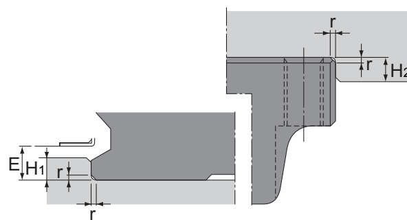
Shoulder for the LM Rail
