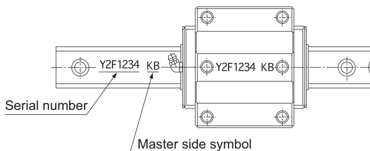
Fig.17 Master LM Rail
