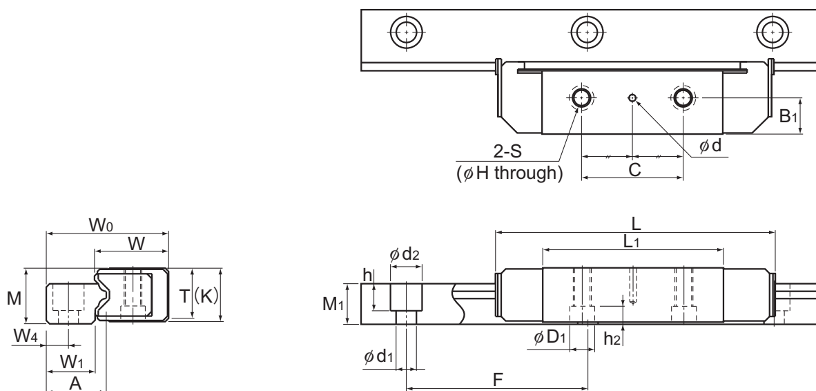
Models HR1123 to 2555M/T/TM
