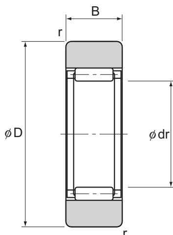
Model RNAST
