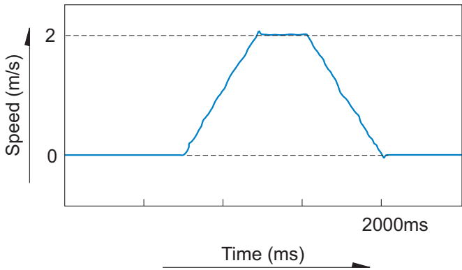
Fig.7 Velocity diagram
