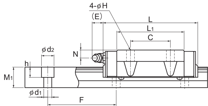
Model SR-M1TB
