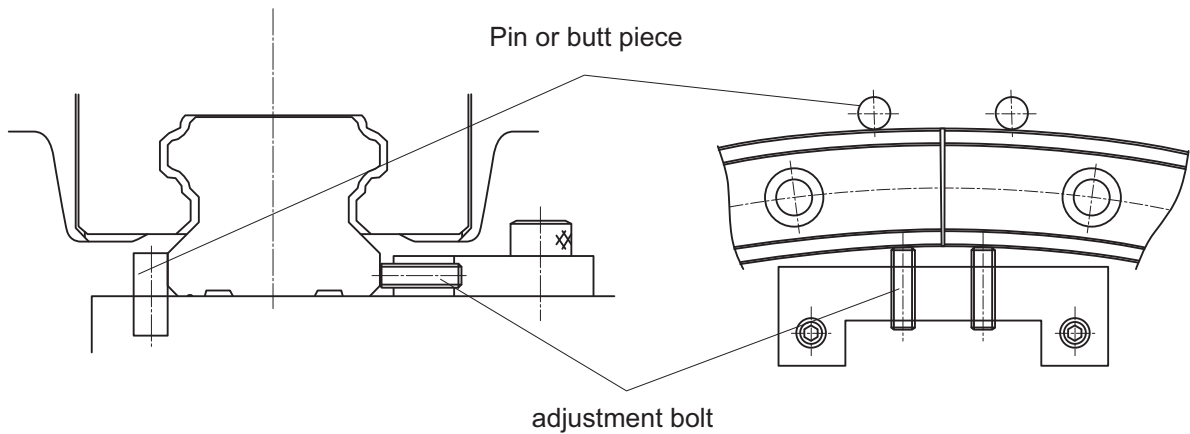
Fig.1 Flush piece
