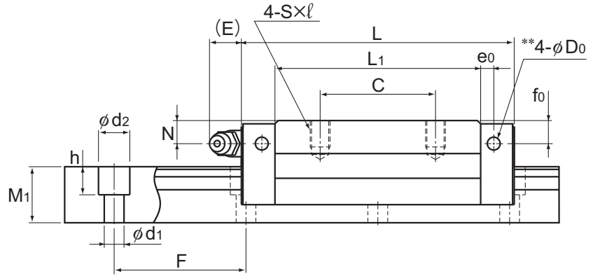
Model NRS-R
