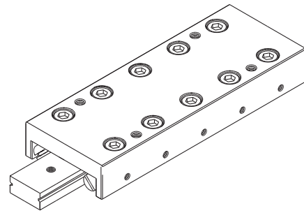
Model VRT
