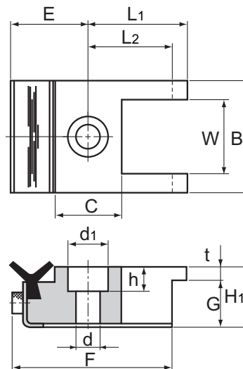
Model SEB
