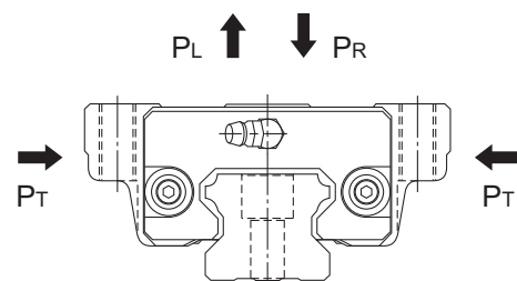
Fig.1 Model HSR-M2
