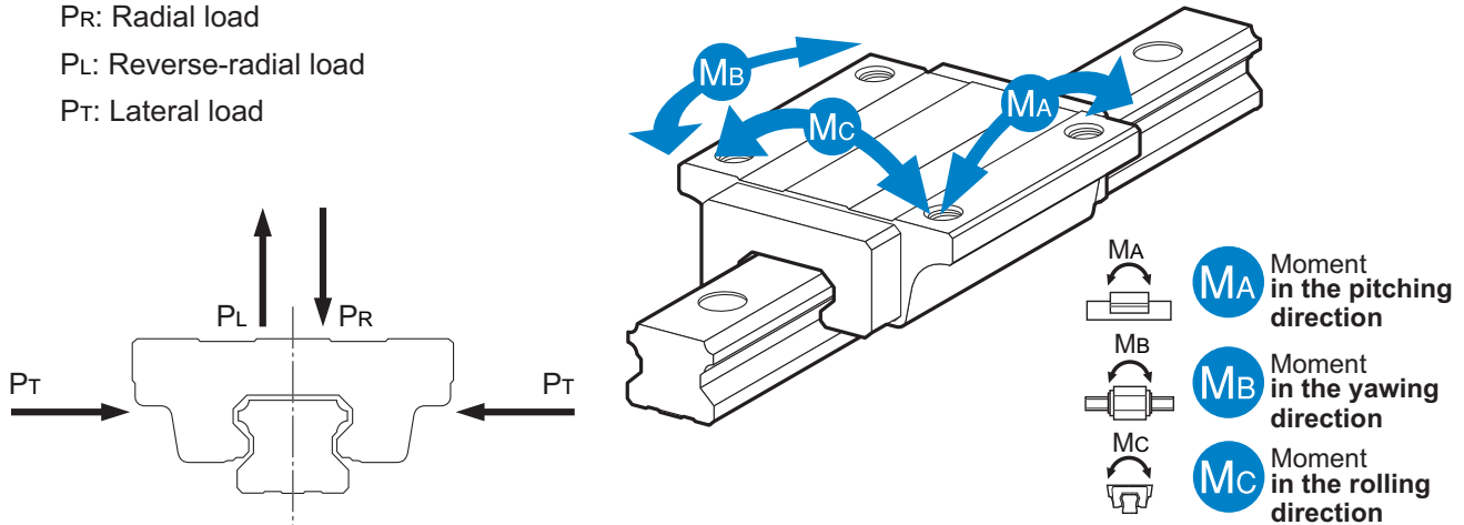
Fig.9 Directions of the Loads Applied on the LM Guide
