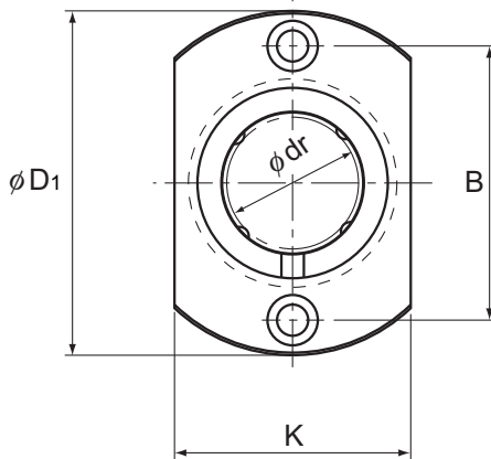
Models LMH6 to 13
