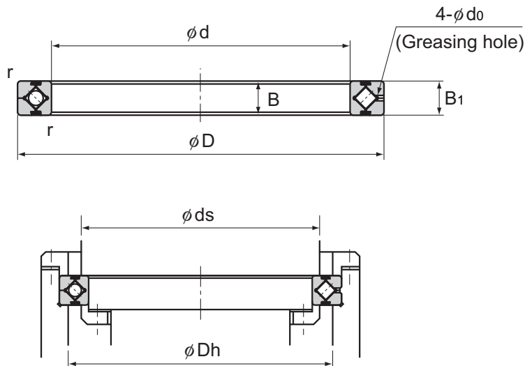
Model RA...CUU
