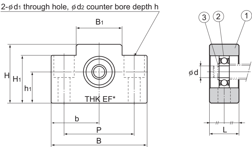
Models EF 6 and 8
