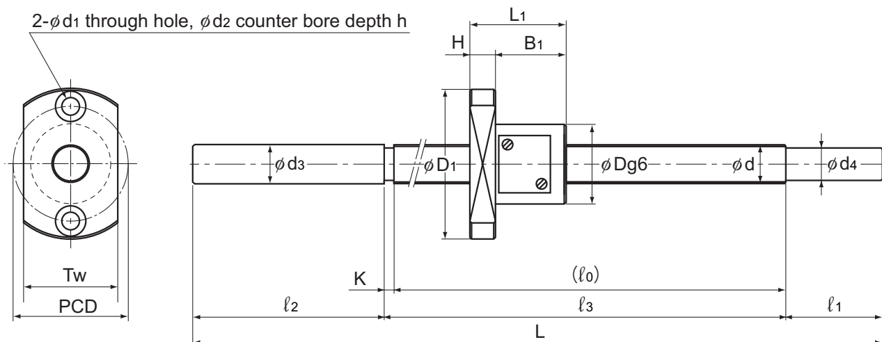
Model MBF
