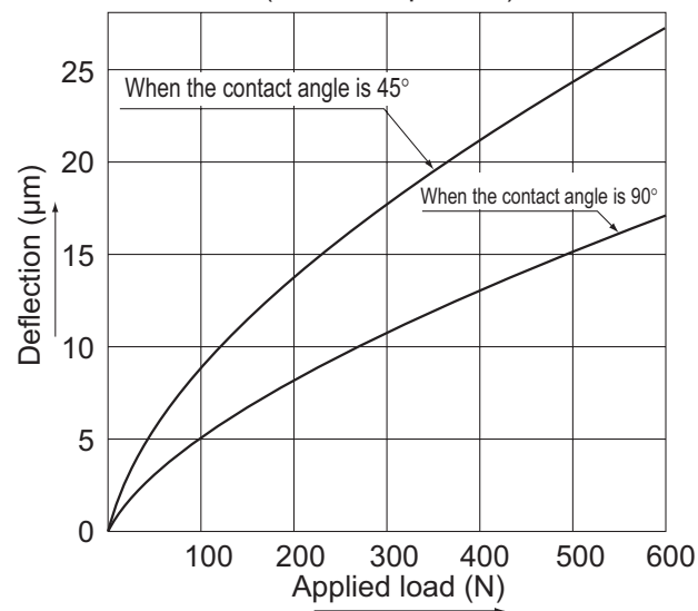
Fig.4 Radial Load and Deflection
