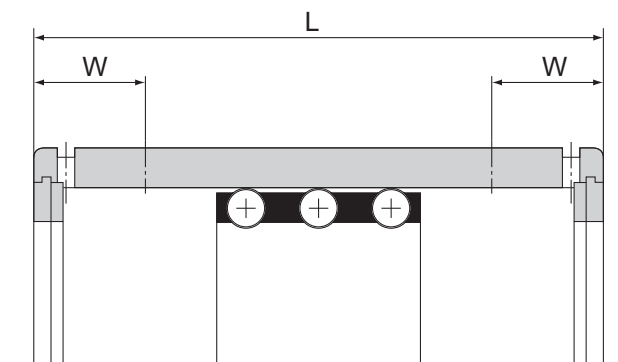
Fig.4 Measurement Range of the Nut
