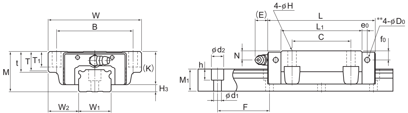
Model NR-B
