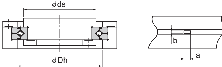
Detail view of the greasing hole
