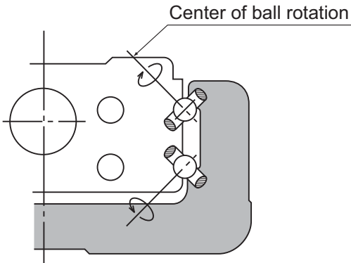
Fig.4 Contact Structure of SKR
