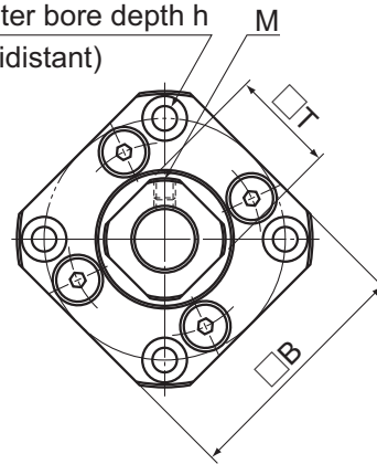
Models FK 10 to 30
