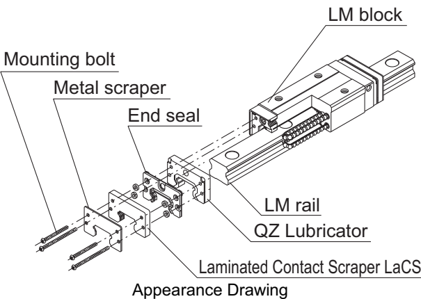
Appearance Drawing
