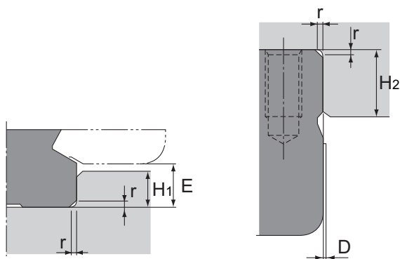
Shoulder for the LM Rail
