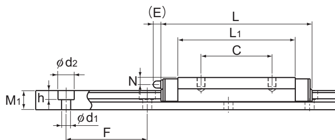
Models RSR14WV and 15WV/WVM/WN
