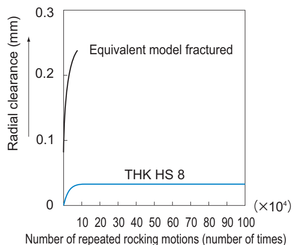
Fig.2 Wear Diagram
