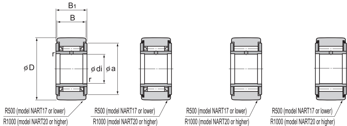
Model NART-R
