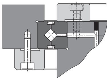
a. Outer ring rotating in the swiveling unit
