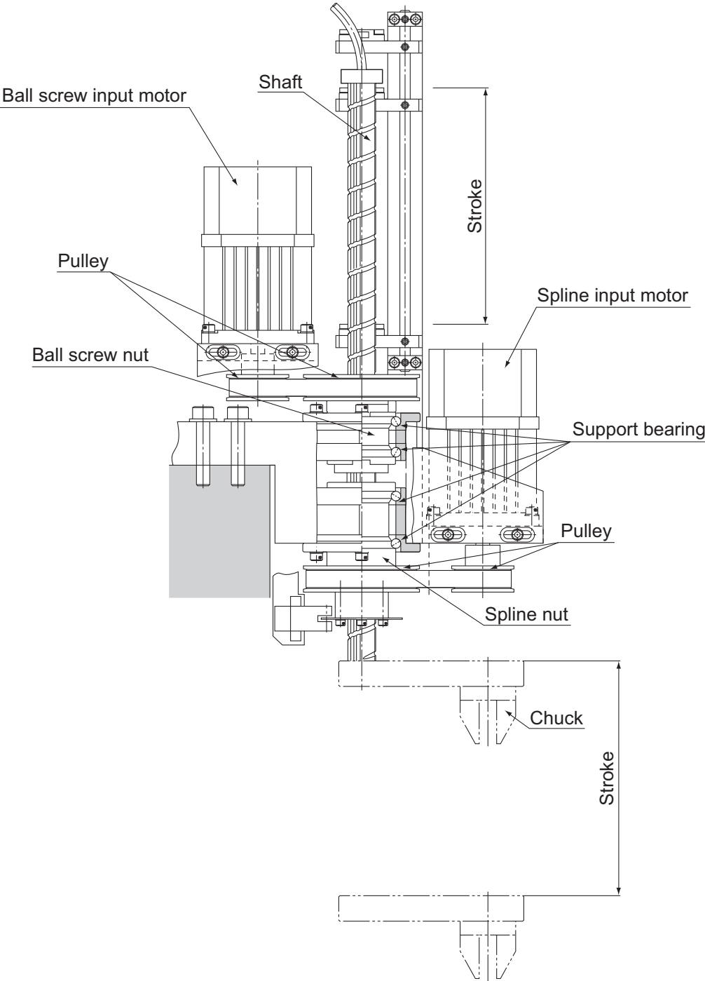
Fig.5 Example of Using Model BNS
