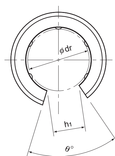
Model LM-OP
