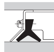
Fig.2 Reinforced Wiper
