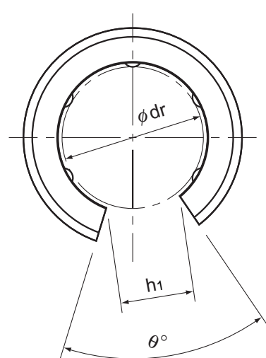
Model LME-OP
