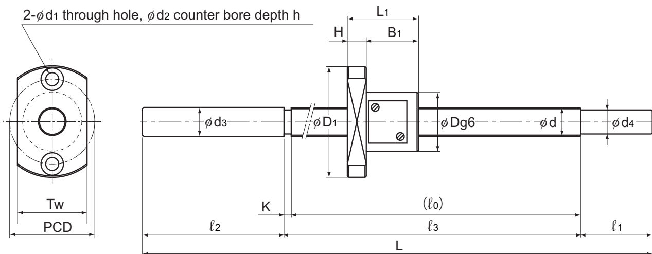
Model MBF
