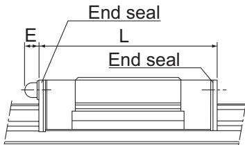
Fig.2 Dimensions of the Grease Nipple for Model SRS
