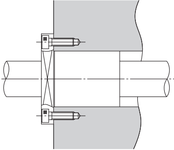
Nut mounted via socket and spigot joint
