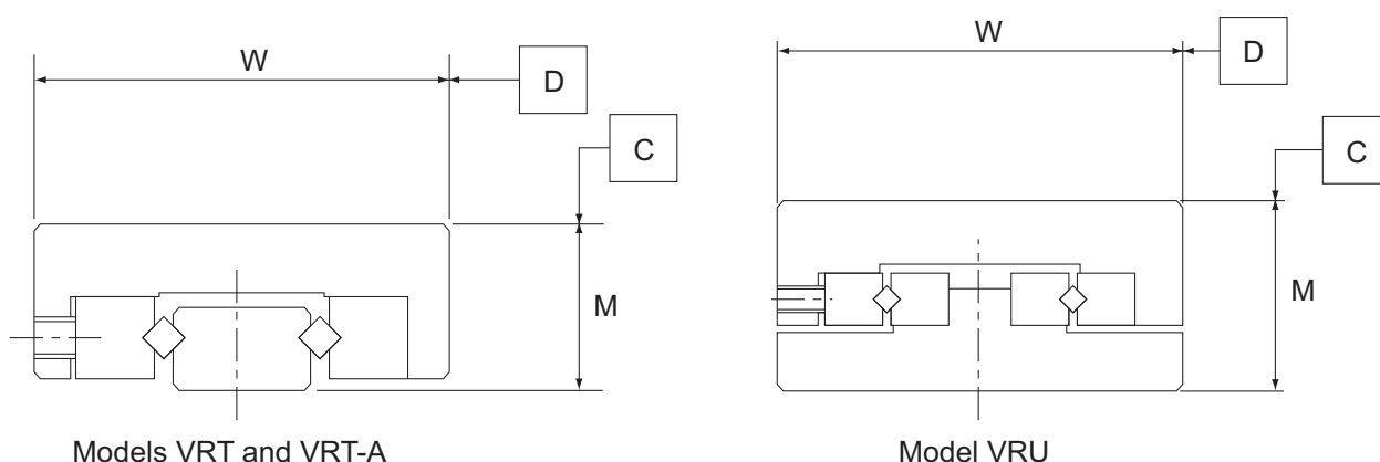
Fig.2 Accuracy Standards
