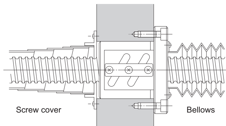
Fig.1 Contamination Protection Cover
