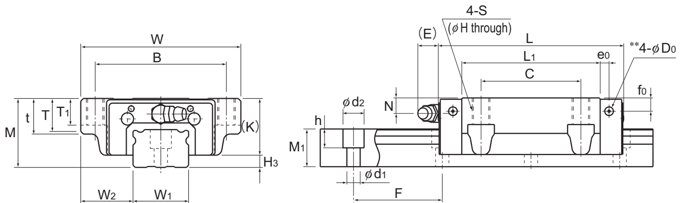
Model SNS-C
