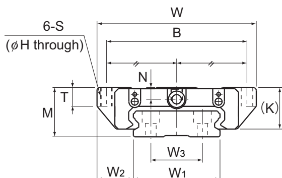
Models SHW17CAM and SHW21 to 50CA
