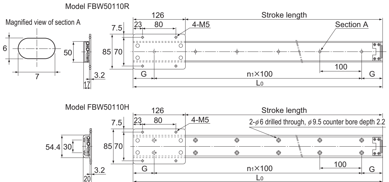
[Models FBW 50110R and 50110H]
