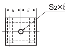
Top surface of models SH3 to SH5
