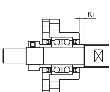
Model FK
