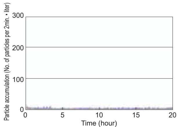
Caged Ball LM Guide Model SSR20
