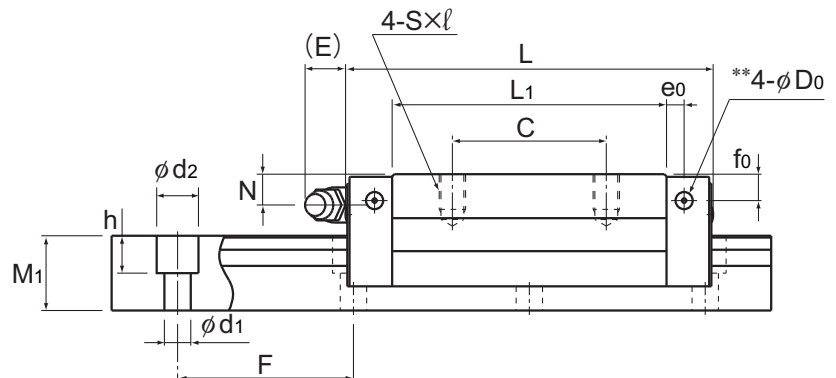
Model SNR-R
