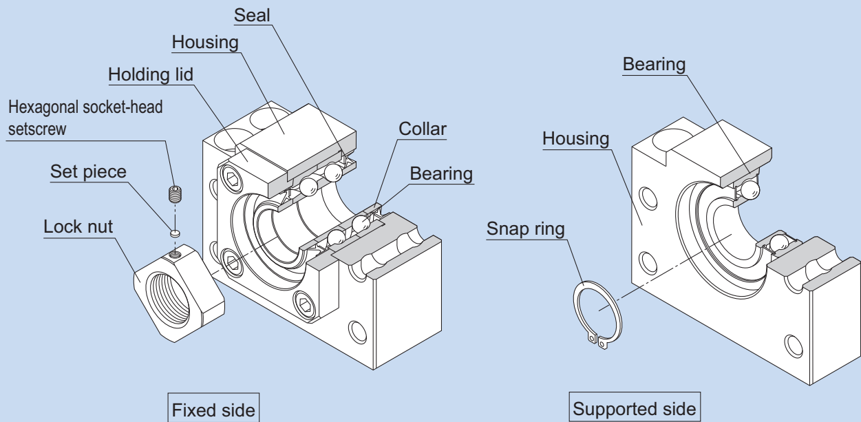
Fig.1 Structure of the Support Unit
