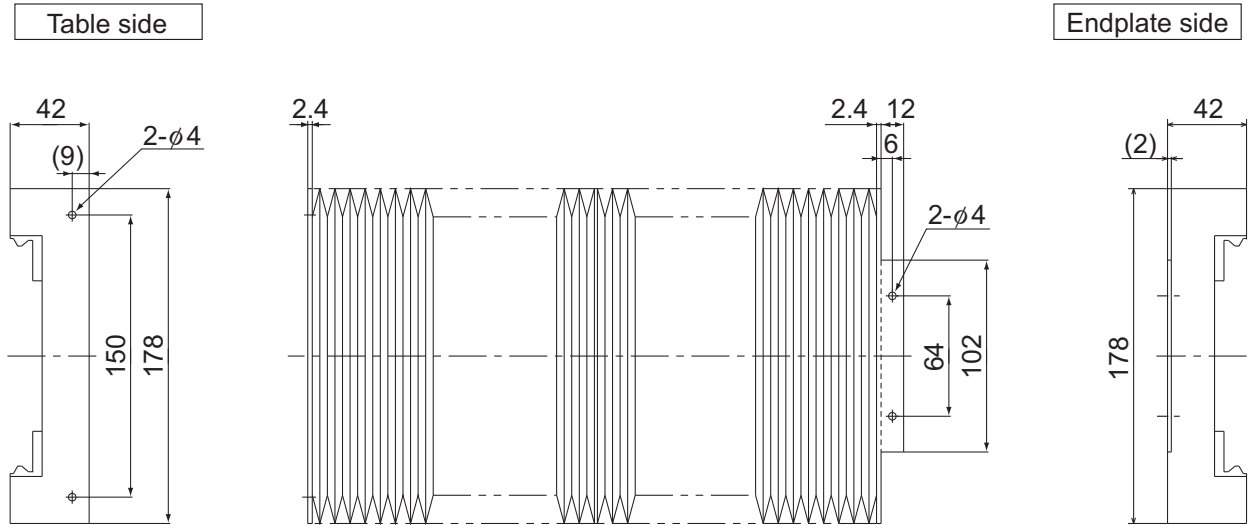
Fig.4 External Dimensions of the Bellows
