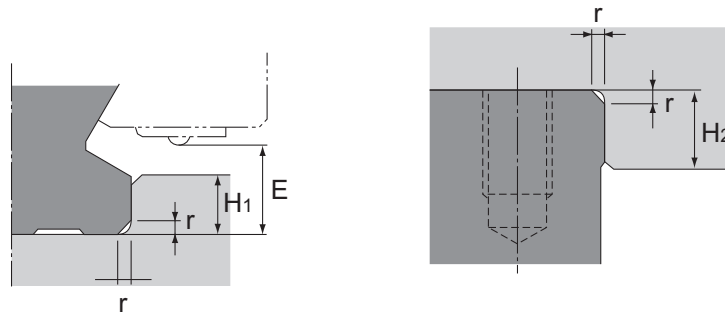
Shoulder for the LM Rail
