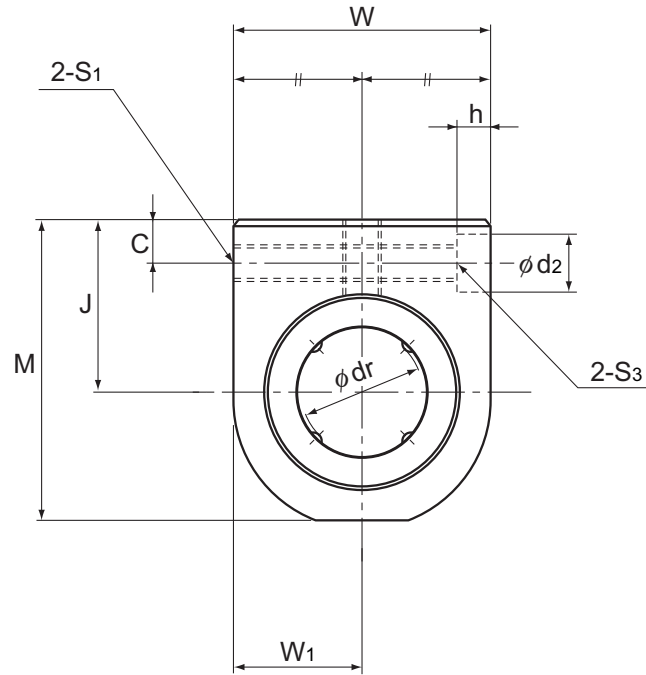
Model SH-L
