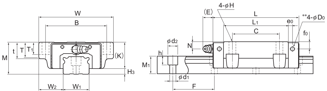
Model NRS-B
