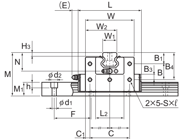
Models CSR20 to 45
