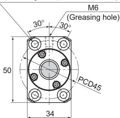
X-X arrow view
