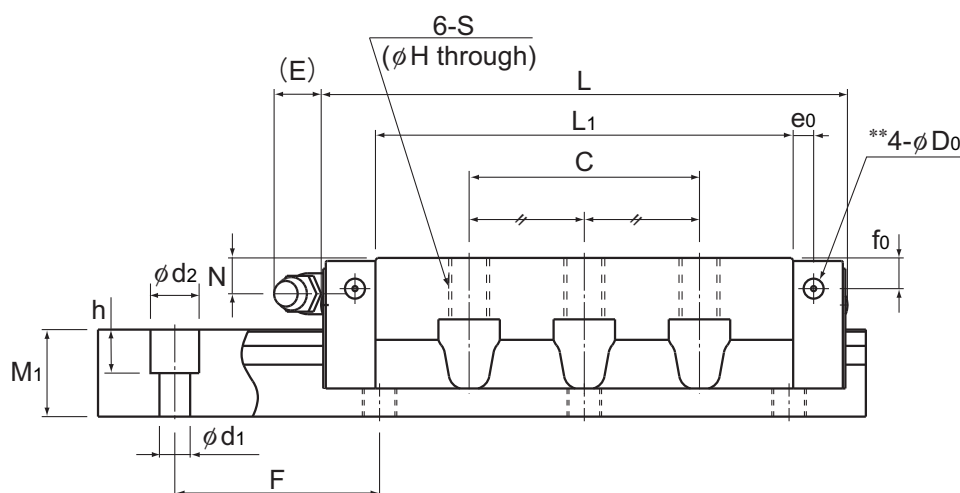
Model SNR-LC
