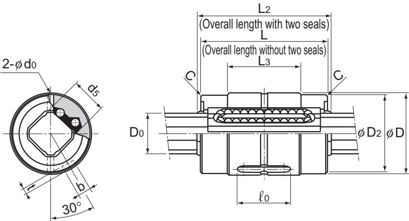
Models LBS6 and 8
