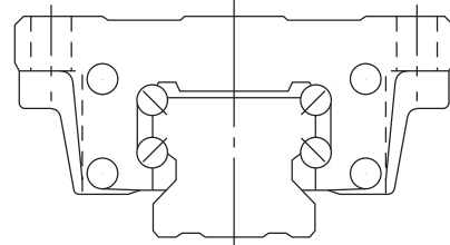
DF Type Four-row Angular Contact (LM Guide)
