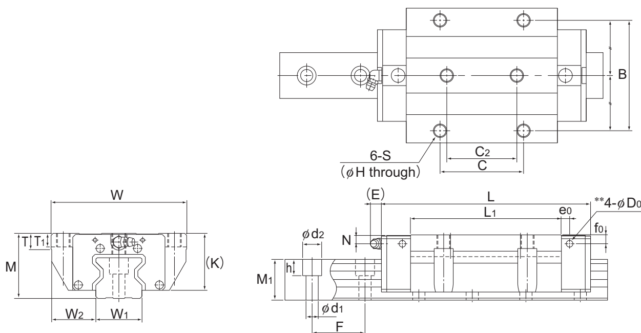
Models SRG25 to 65C/LC
