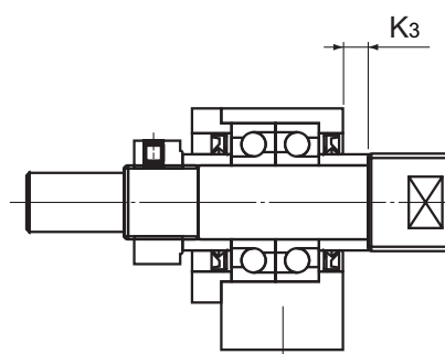
Model EK
