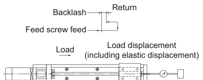
Fig.11 Backlash
