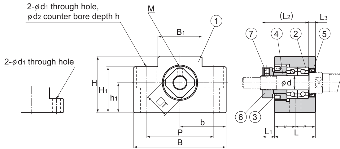
Models EK 4 and 5
