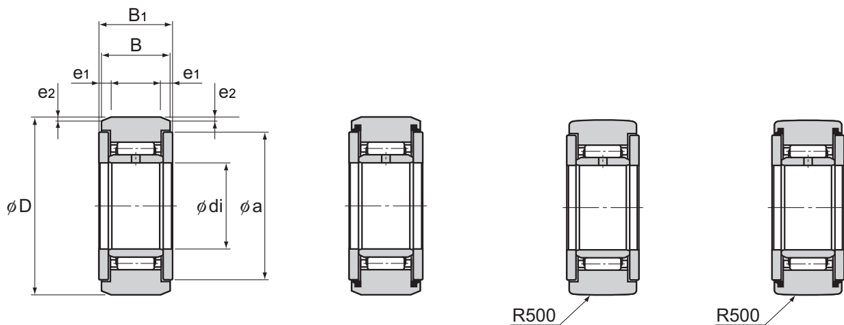
Model NAST-ZZ
