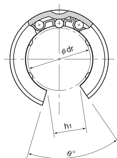
Model LM-GA-OP
