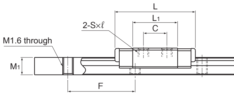
Model RSR3M
