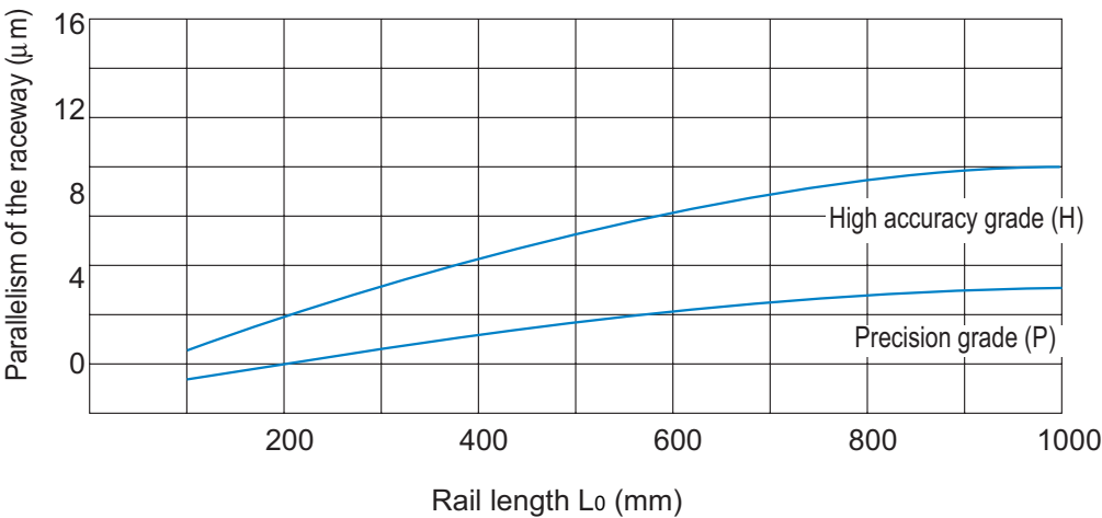
Fig.4 Rail Length and Parallelism of the Raceway
