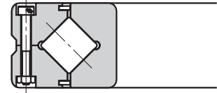
Model RB
