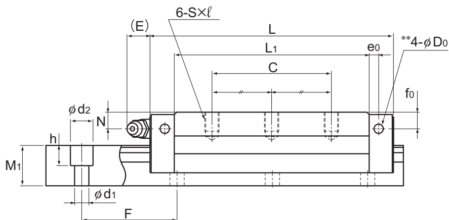
Model NRS-LR
