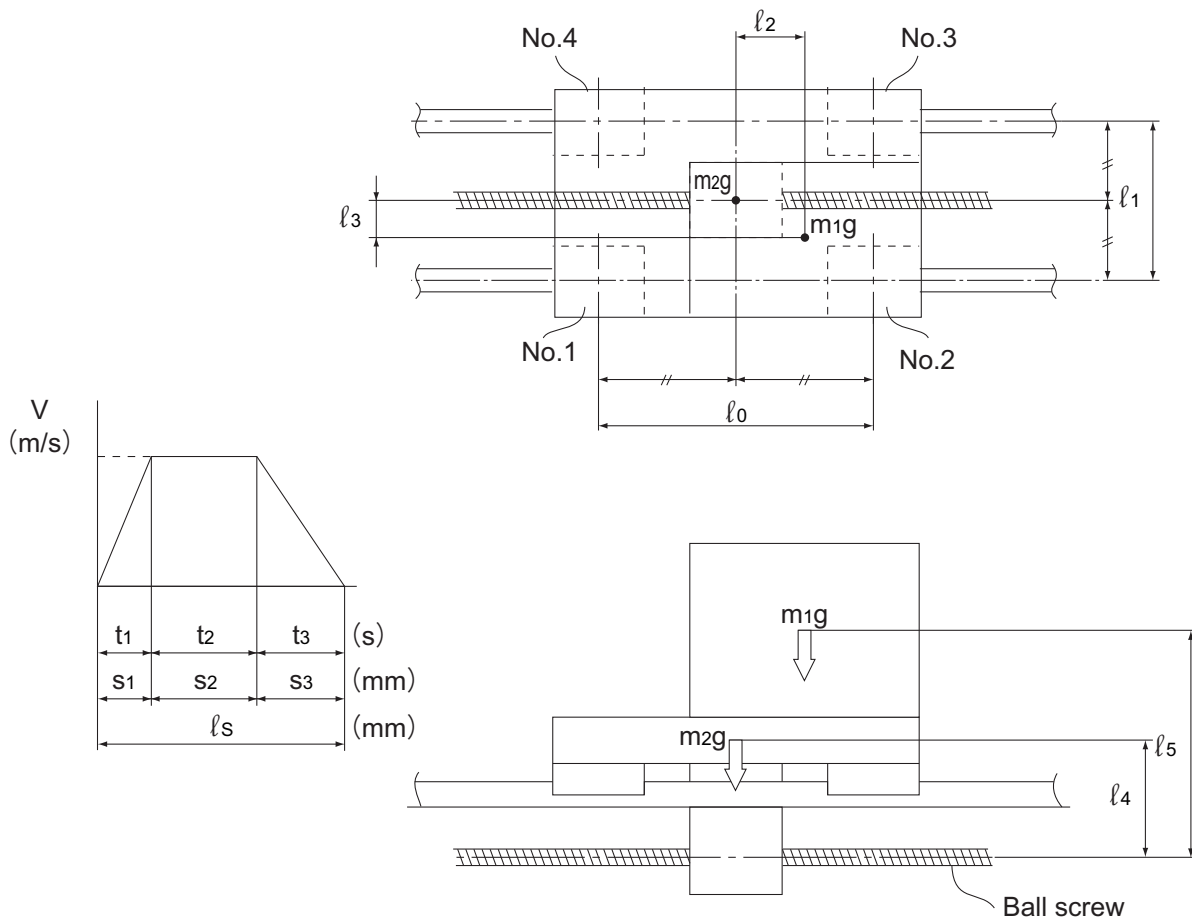
Fig.13 Condition
