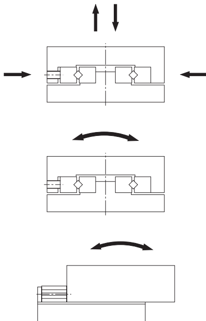
Fig.2 Load Directions
