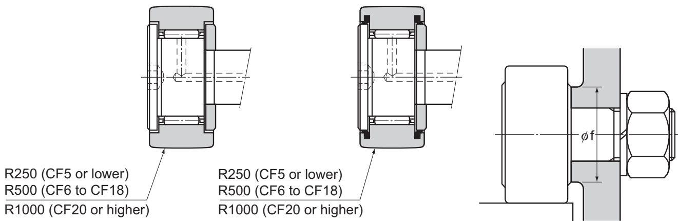
Model CF-R-A
