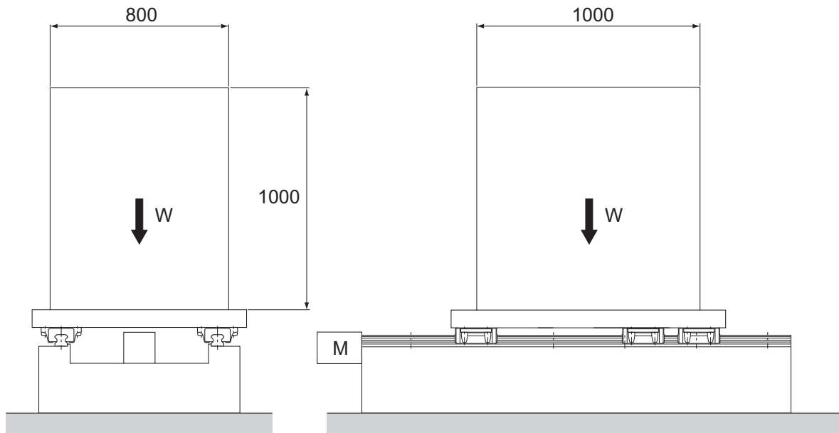
Fig.6 Condition
