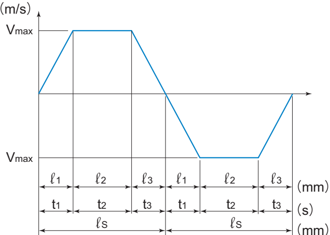
Velocity diagram
