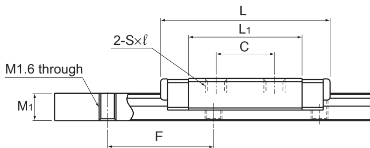
Model RSR3N
