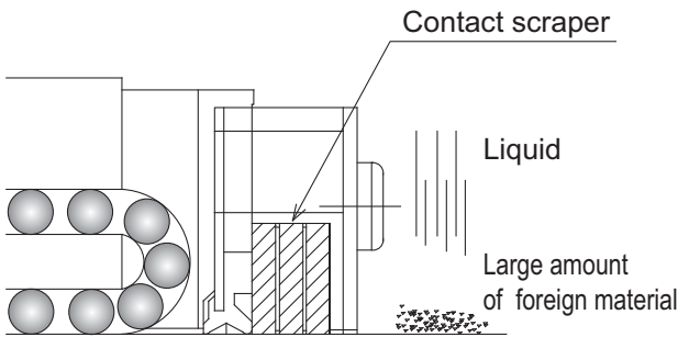
Structural Drawing
