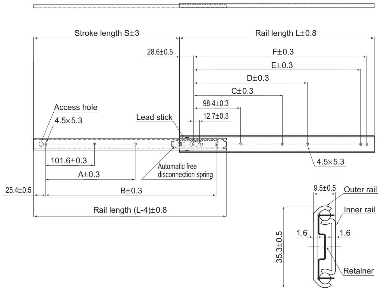
Cross section
