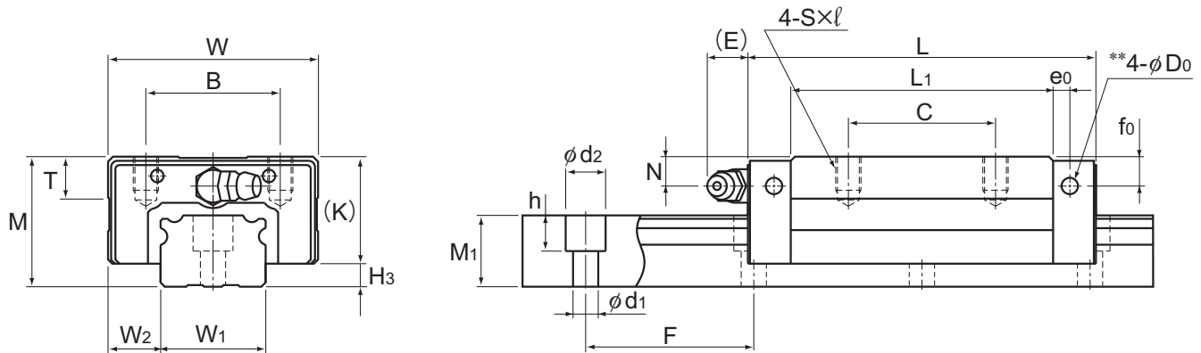
Model NR-R
