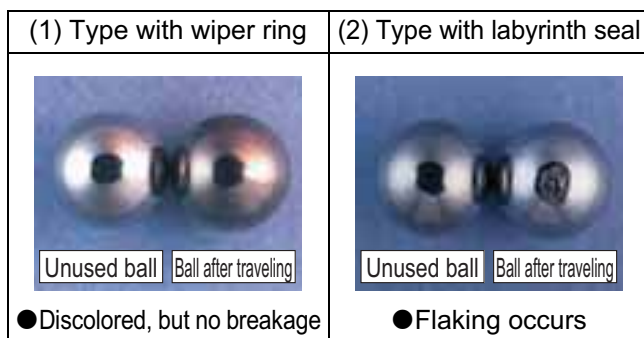
Change in the ball after traveling 2000 km
