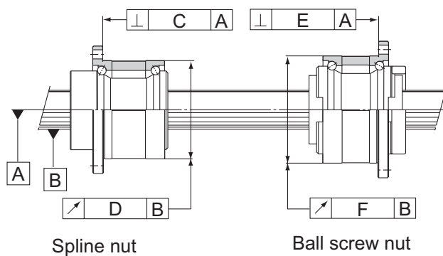
Model BNS
