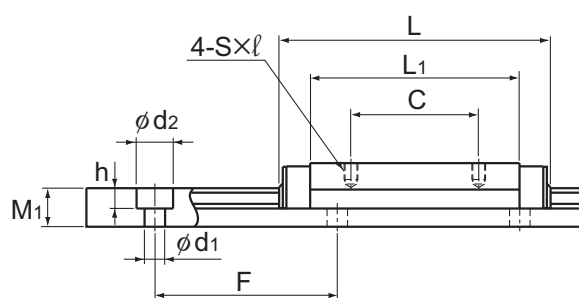
Models RSR9 and 12WV/WVM/WN
